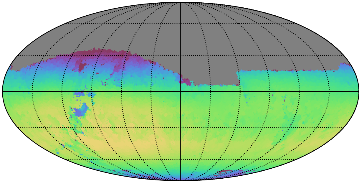
too_elab_r8_d3_griz_v3.4_10yrs Yr 1 i band: Max skyBrightness
