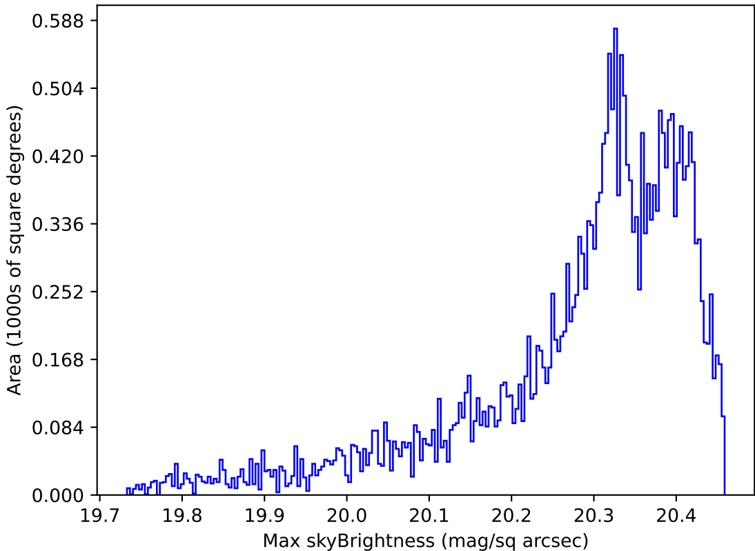
too_elab_r8_d3_griz_v3.4_10yrs Yr 1 i band: Max skyBrightness
