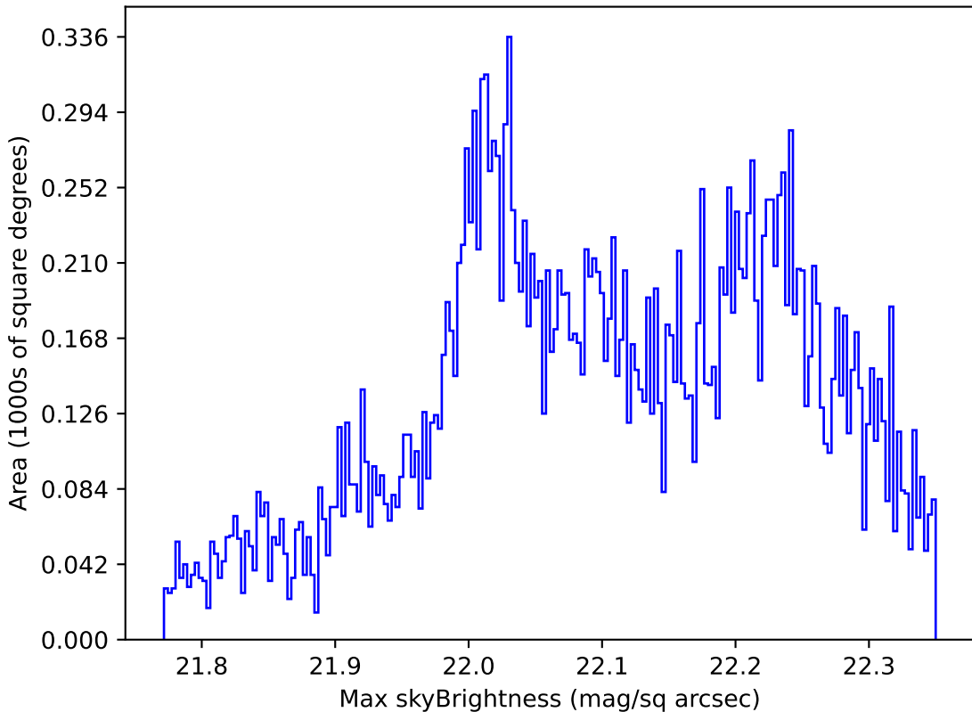
too_elab_r8_d3_griz_v3.4_10yrs Yr 1 g band: Max skyBrightness
