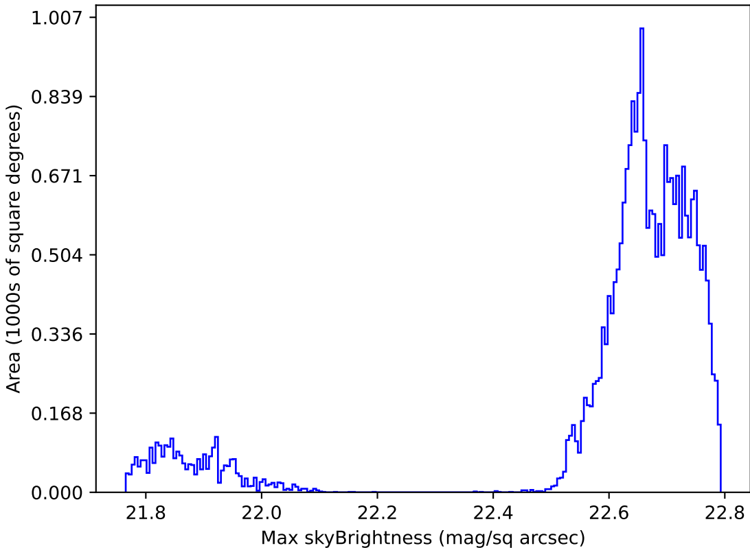
too_elab_r8_d3_griz_v3.4_10yrs Yr 1 all bands: Max skyBrightness
