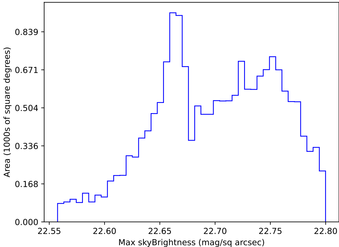
too_elab_r8_d3_griz_v3.4_10yrs WFD u band: Max skyBrightness
