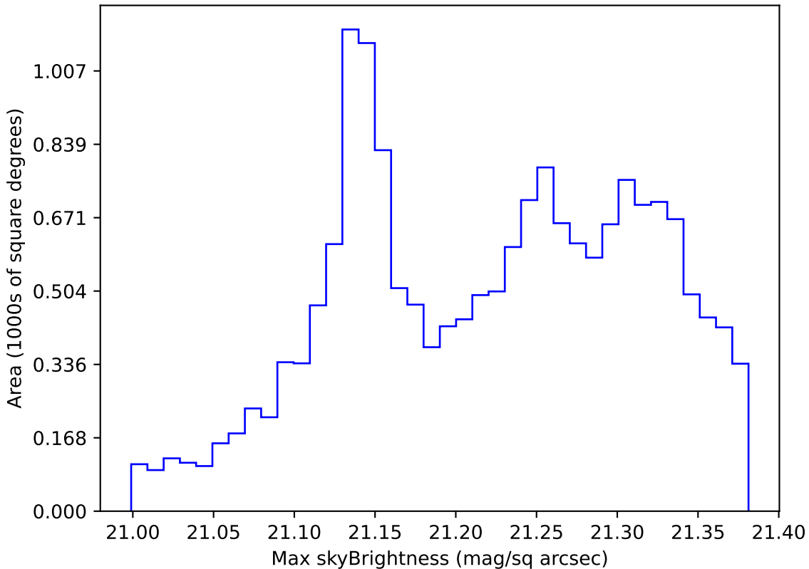
too_elab_r8_d3_griz_v3.4_10yrs WFD r band: Max skyBrightness
