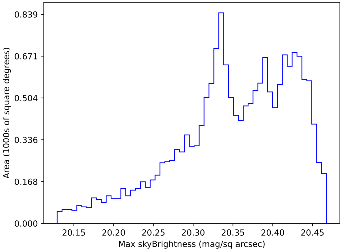
too_elab_r8_d3_griz_v3.4_10yrs WFD i band: Max skyBrightness
