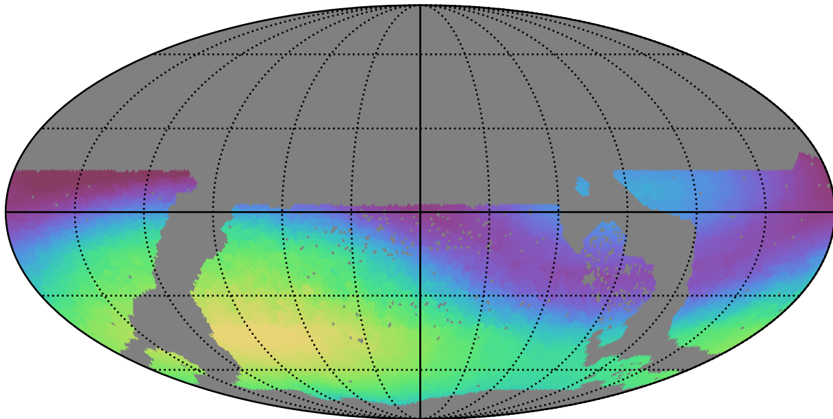
too_elab_r8_d3_griz_v3.4_10yrs WFD g band: Max skyBrightness
