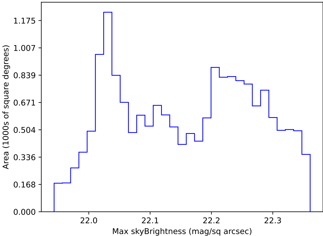
too_elab_r8_d3_griz_v3.4_10yrs WFD g band: Max skyBrightness
