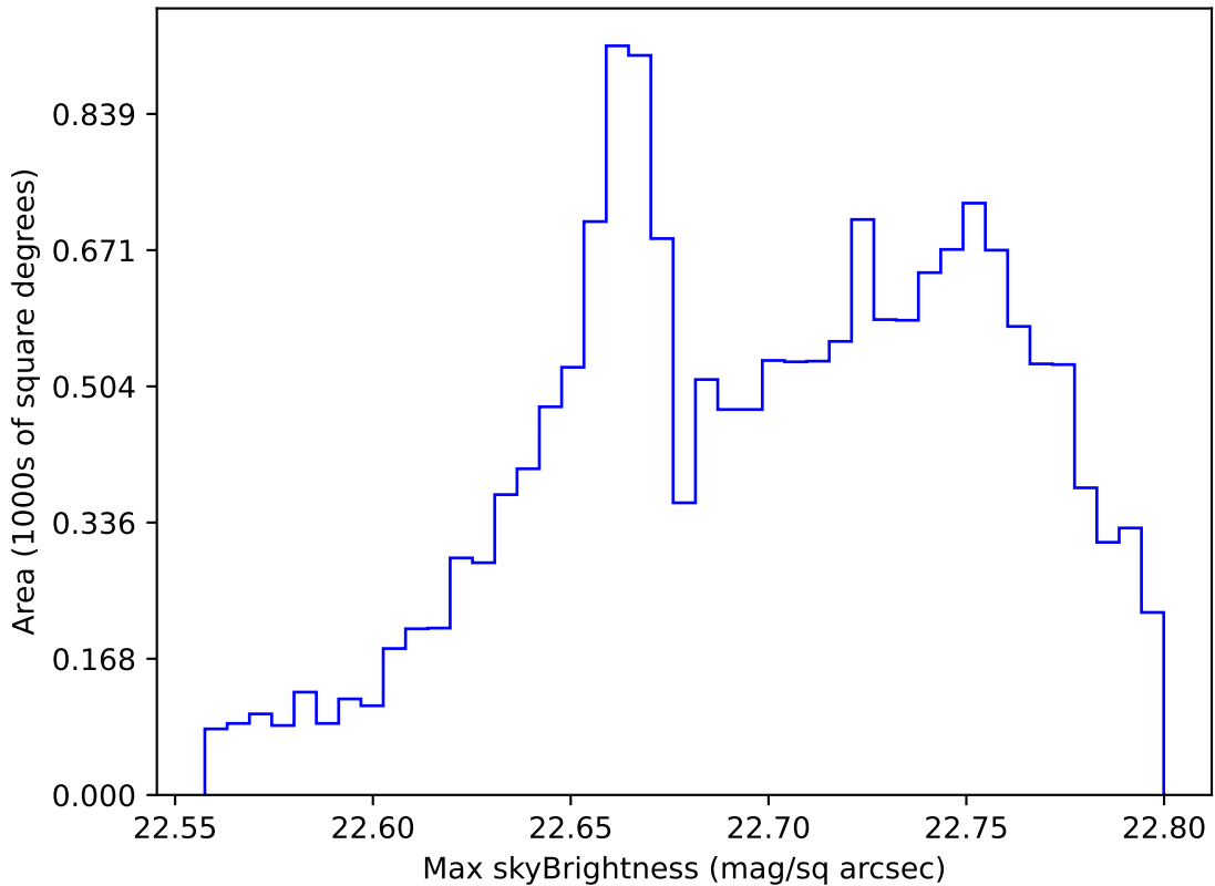
too_elab_r8_d3_griz_v3.4_10yrs WFD all bands: Max skyBrightness
