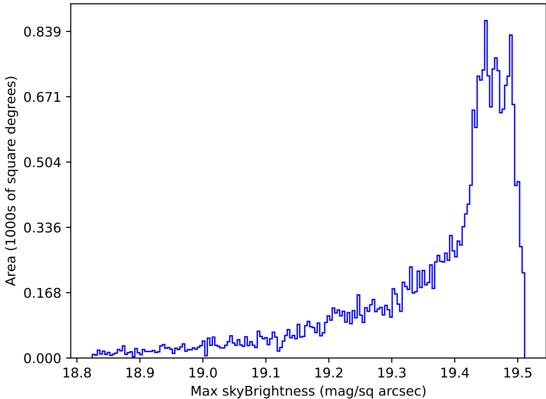
too_elab_r8_d3_griz_v3.4_10yrs All sky z band: Max skyBrightness
