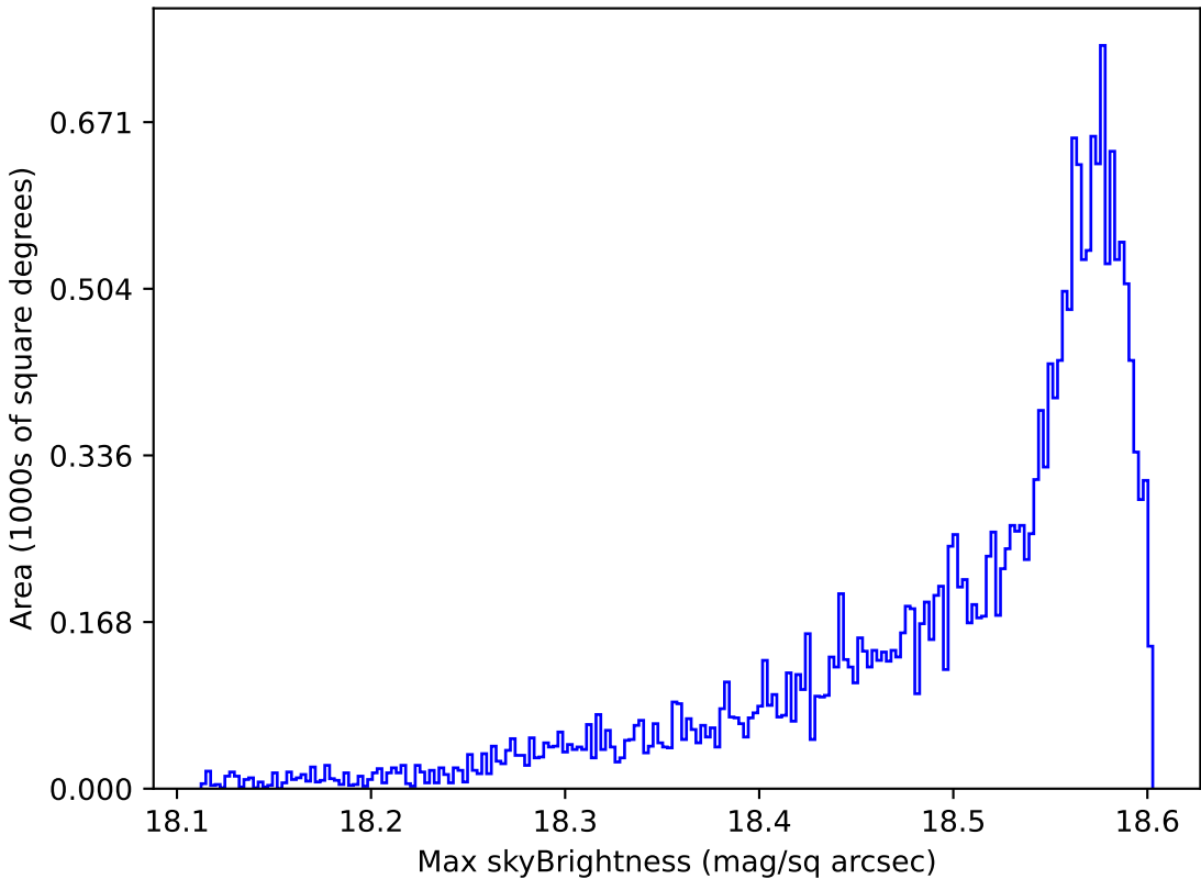
too_elab_r8_d3_griz_v3.4_10yrs All sky y band: Max skyBrightness
