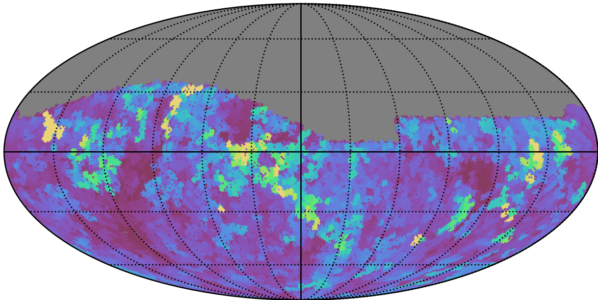
too_elab_r8_d3_griz_v3.4_10yrs Yr 1 z band: Max seeingGeom
