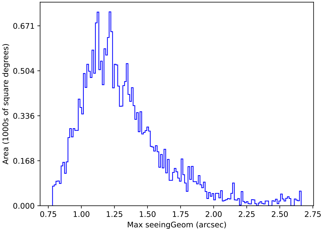
too_elab_r8_d3_griz_v3.4_10yrs Yr 1 z band: Max seeingGeom
