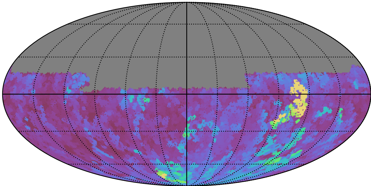
too_elab_r8_d3_griz_v3.4_10yrs Yr 1 u band: Max seeingGeom
