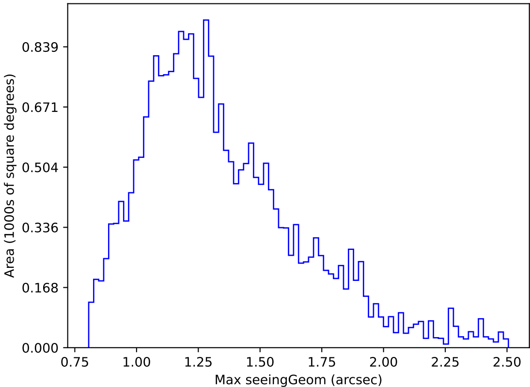
too_elab_r8_d3_griz_v3.4_10yrs Yr 1 i band: Max seeingGeom
