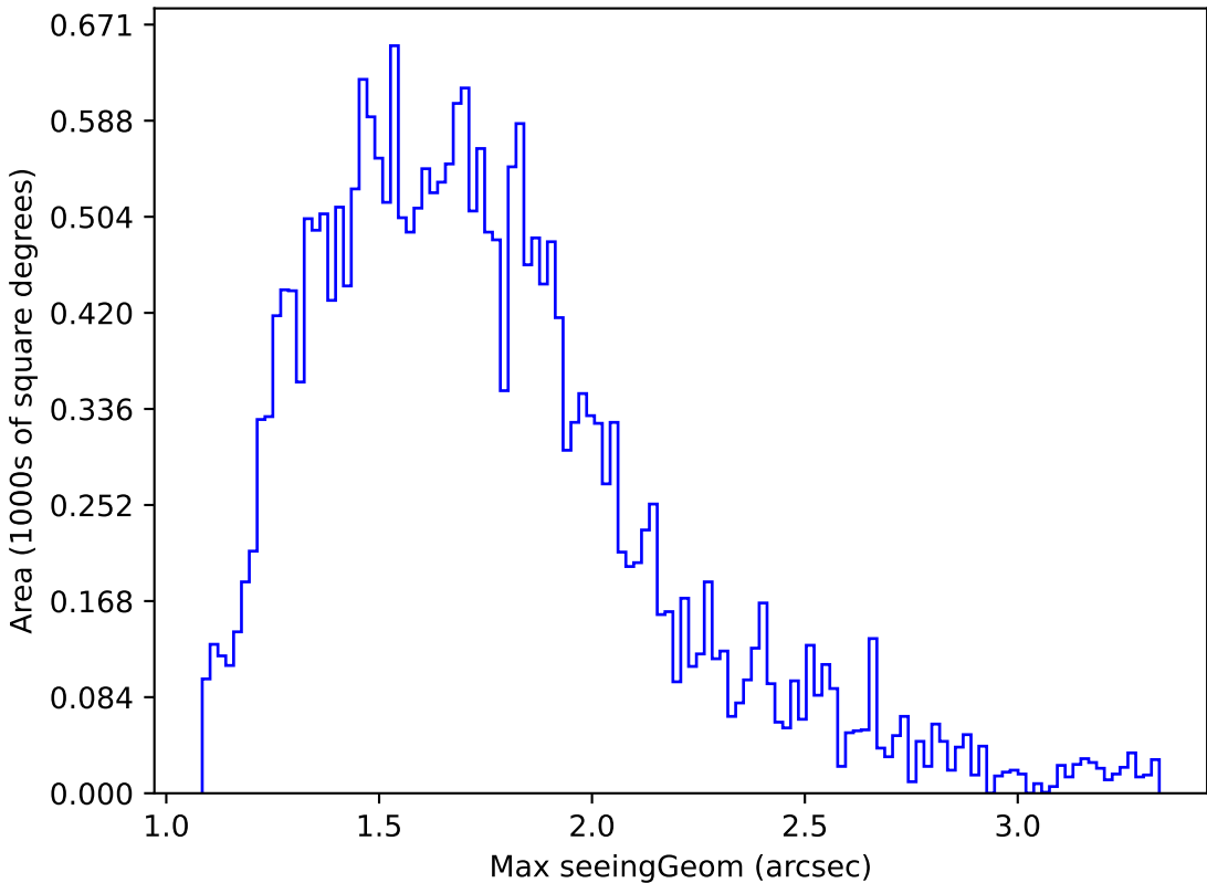
too_elab_r8_d3_griz_v3.4_10yrs Yr 1 all bands: Max seeingGeom
