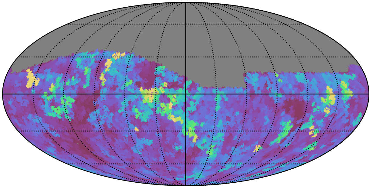
too_elab_r8_d3_griz_v3.4_10yrs Yr 1 z band: Max seeingEff
