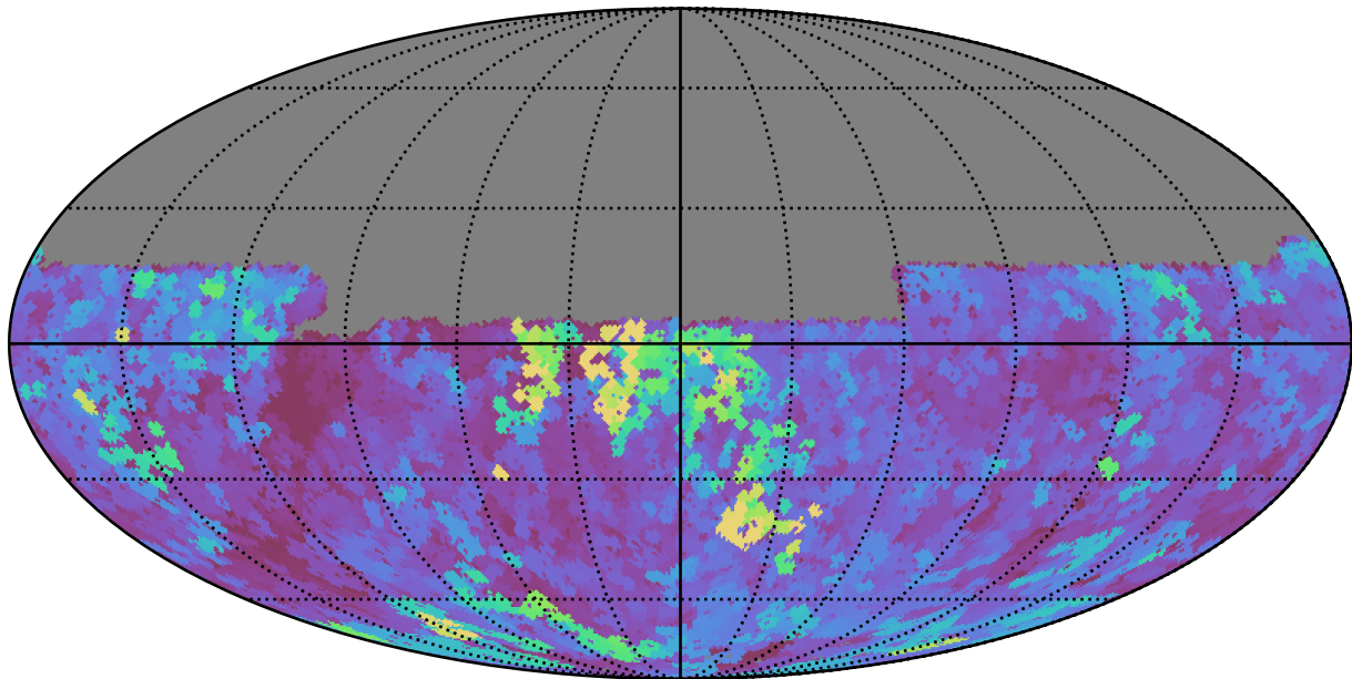
too_elab_r8_d3_griz_v3.4_10yrs Yr 1 y band: Max seeingEff
