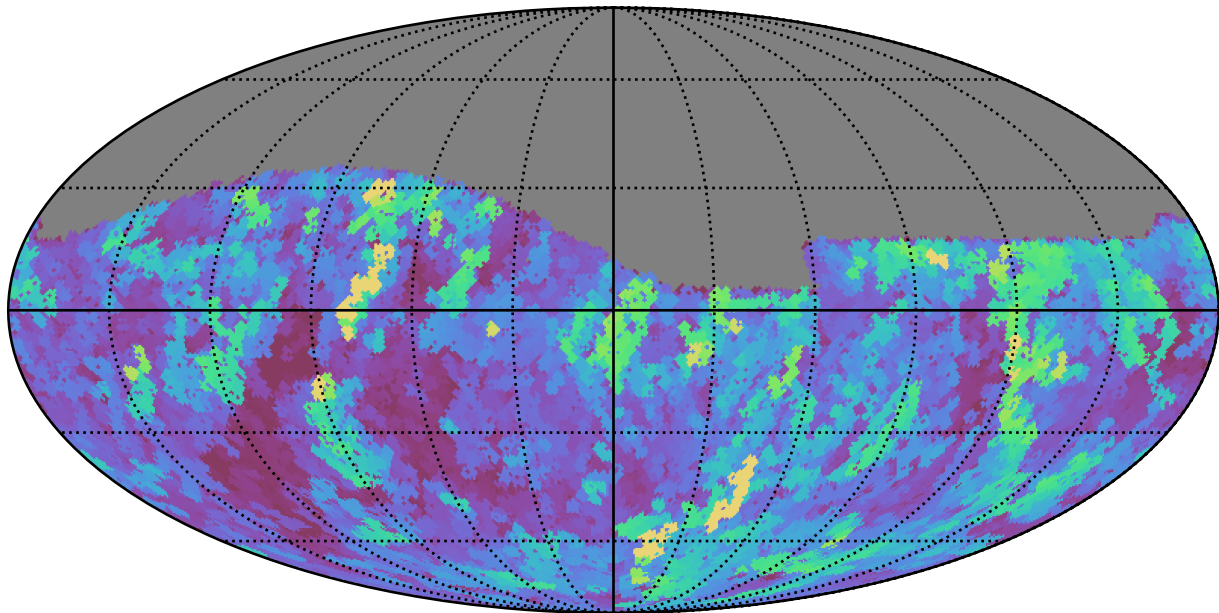
too_elab_r8_d3_griz_v3.4_10yrs Yr 1 r band: Max seeingEff
