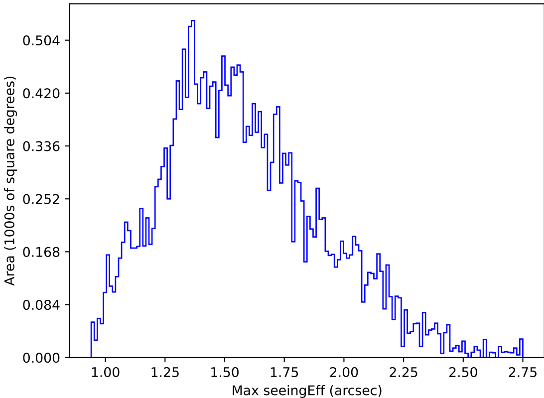
too_elab_r8_d3_griz_v3.4_10yrs Yr 1 r band: Max seeingEff
