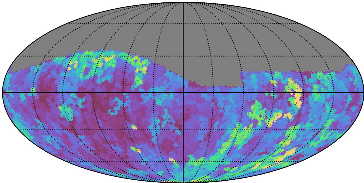
too_elab_r8_d3_griz_v3.4_10yrs Yr 1 g band: Max seeingEff
