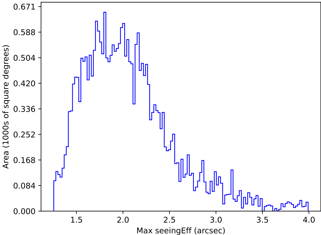
too_elab_r8_d3_griz_v3.4_10yrs Yr 1 all bands: Max seeingEff
