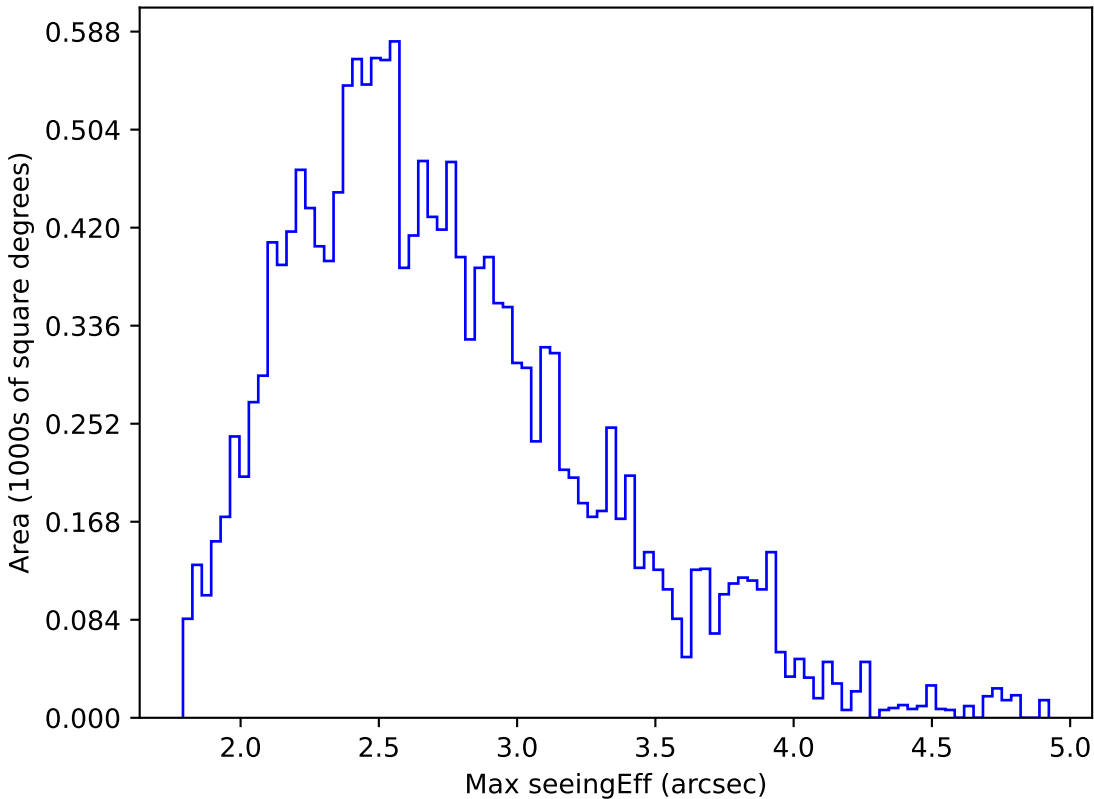
too_elab_r8_d3_griz_v3.4_10yrs WFD r band: Max seeingEff
