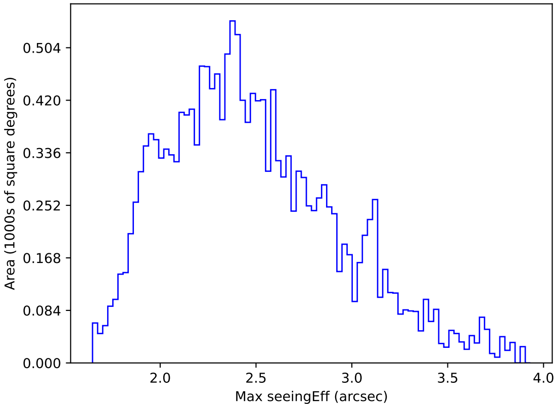
too_elab_r8_d3_griz_v3.4_10yrs WFD g band: Max seeingEff
