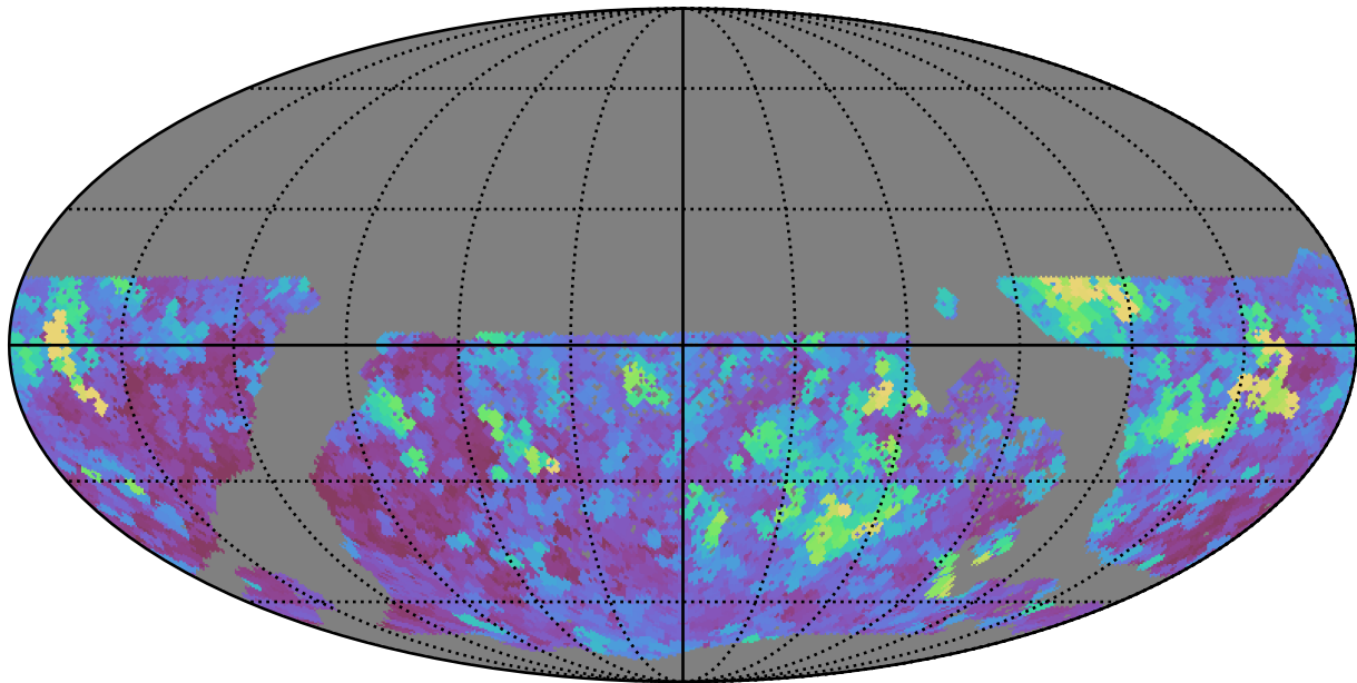
too_elab_r8_d3_griz_v3.4_10yrs WFD all bands: Max seeingEff
