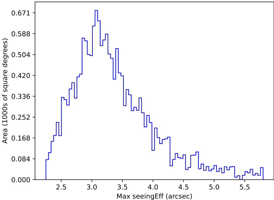
too_elab_r8_d3_griz_v3.4_10yrs WFD all bands: Max seeingEff
