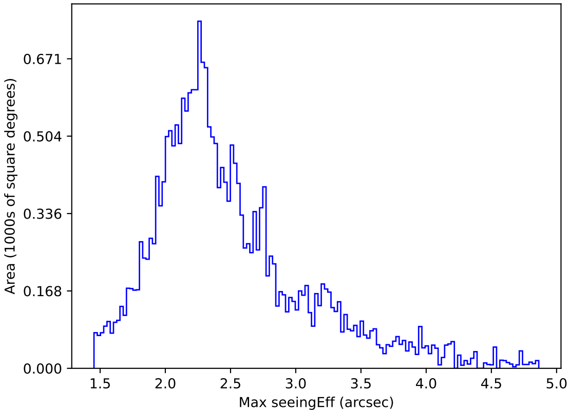
too_elab_r8_d3_griz_v3.4_10yrs All sky u band: Max seeingEff
