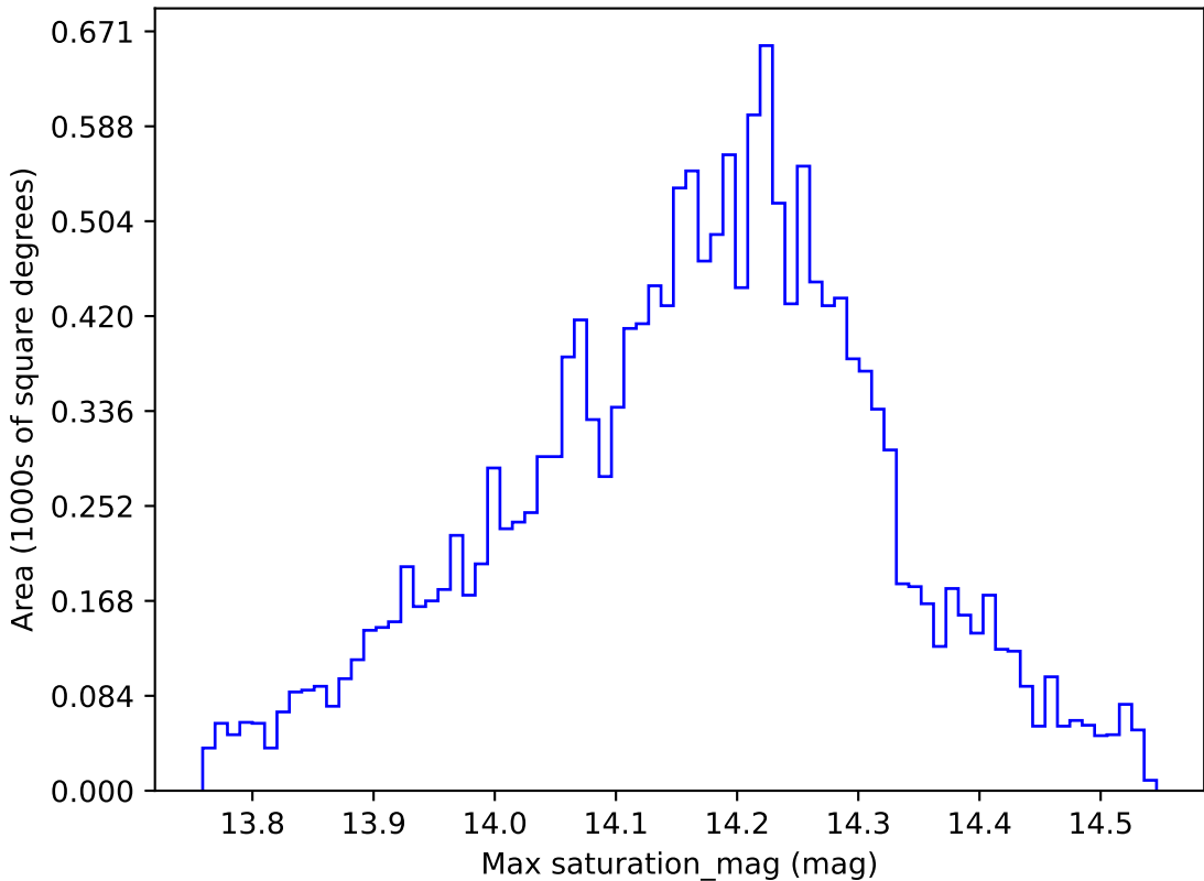
too_elab_r8_d3_griz_v3.4_10yrs WFD y band: Max saturation_mag
