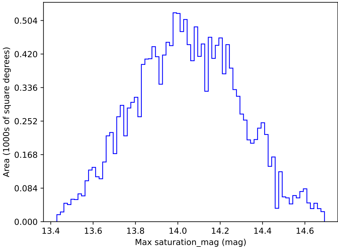
too_elab_r8_d3_griz_v3.4_10yrs WFD u band: Max saturation_mag
