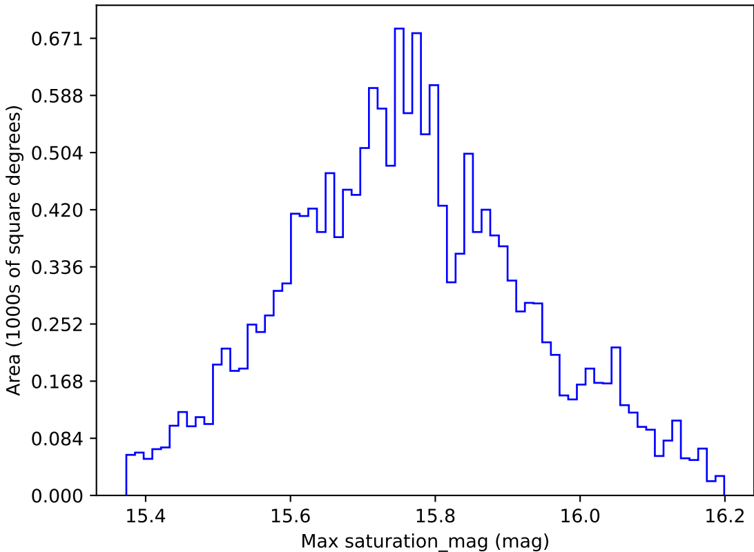
too_elab_r8_d3_griz_v3.4_10yrs WFD r band: Max saturation_mag
