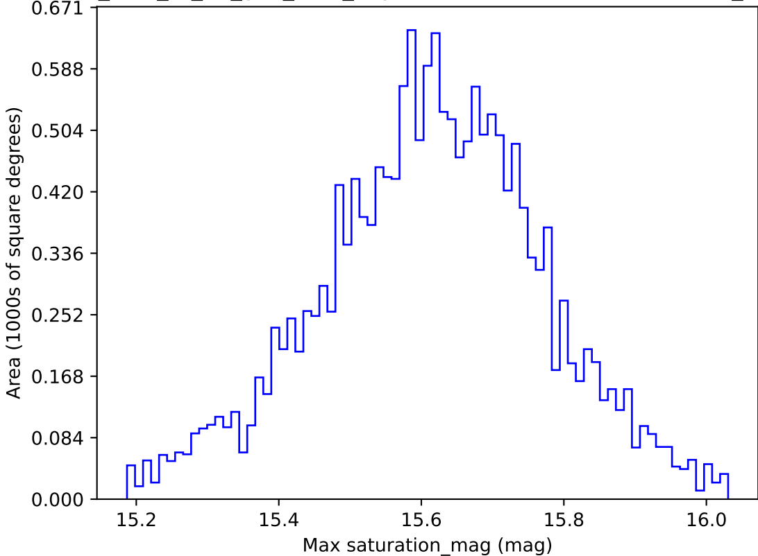
too_elab_r8_d3_griz_v3.4_10yrs WFD i band: Max saturation_mag
