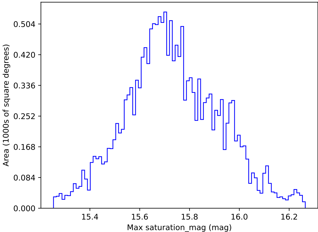
too_elab_r8_d3_griz_v3.4_10yrs WFD g band: Max saturation_mag
