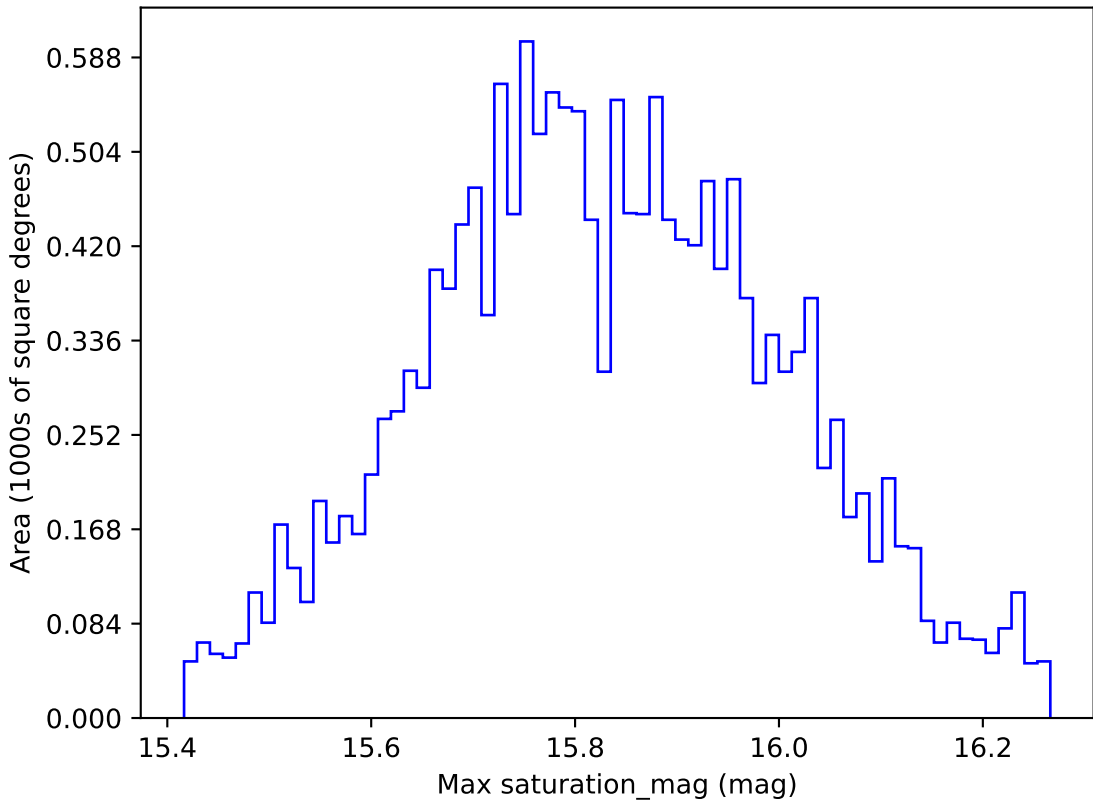
too_elab_r8_d3_griz_v3.4_10yrs WFD all bands: Max saturation_mag
