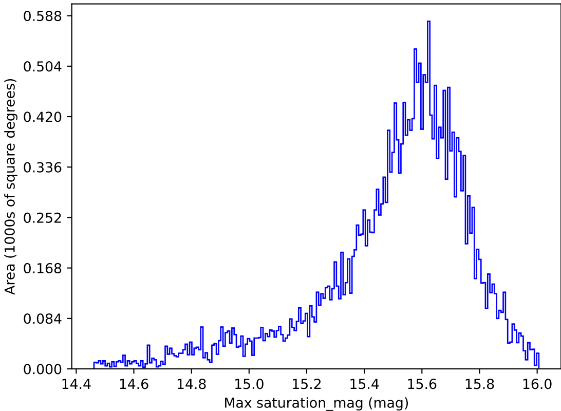
too_elab_r8_d3_griz_v3.4_10yrs All sky i band: Max saturation_mag
