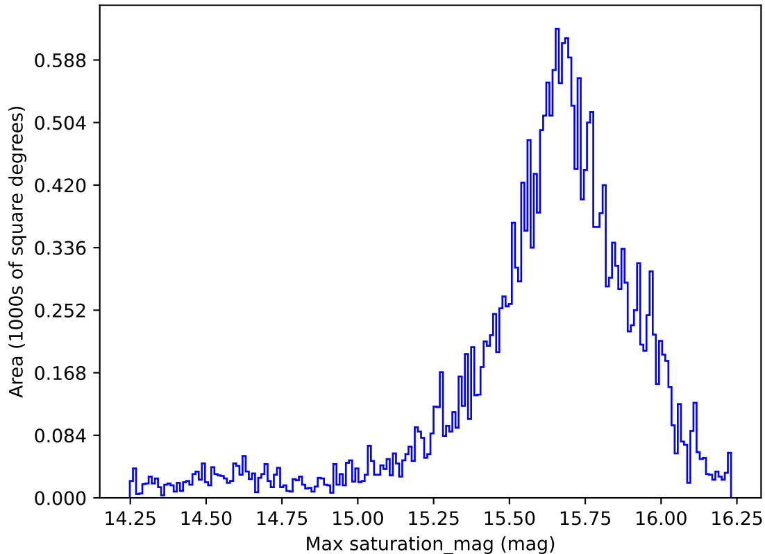
too_elab_r8_d3_griz_v3.4_10yrs All sky g band: Max saturation_mag
