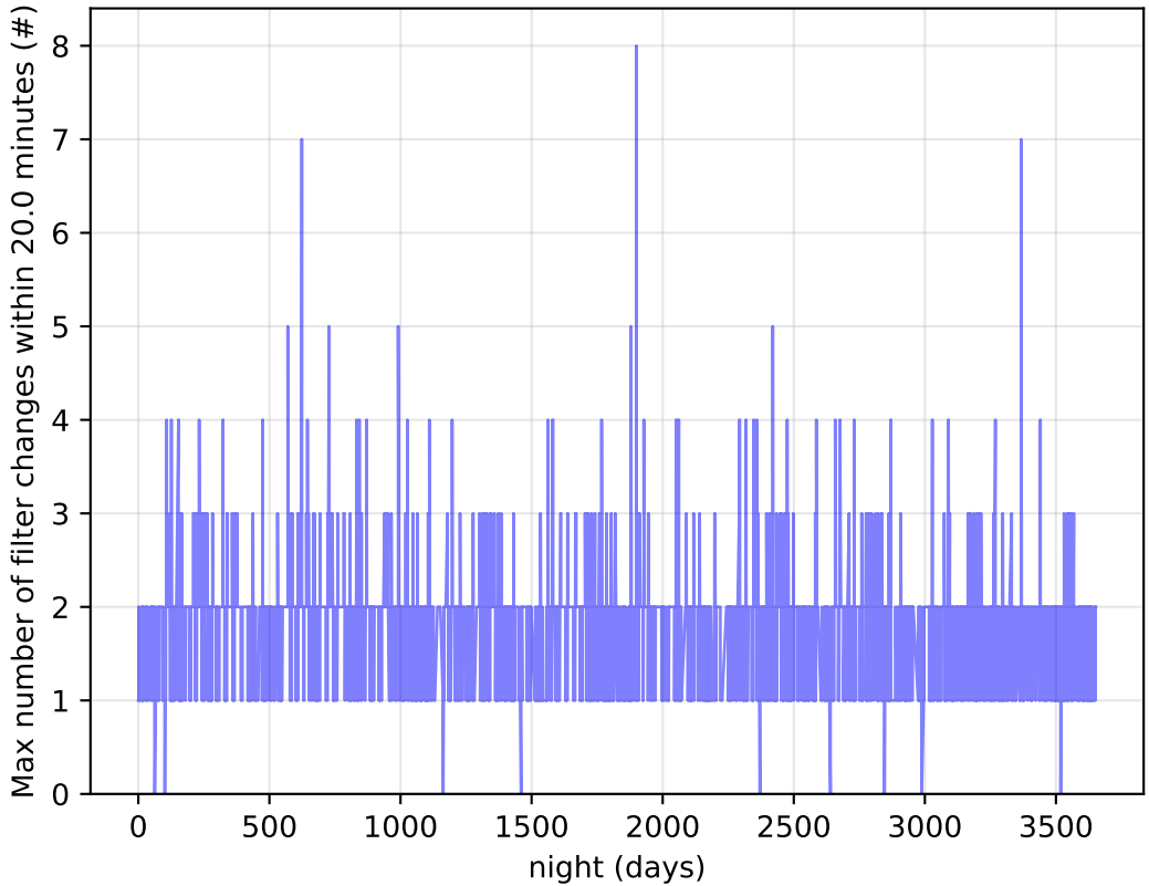
too_elab_r8_d3_griz_v3.4_10yrs Per Night: Max number of filter changes within 20.0 minutes
