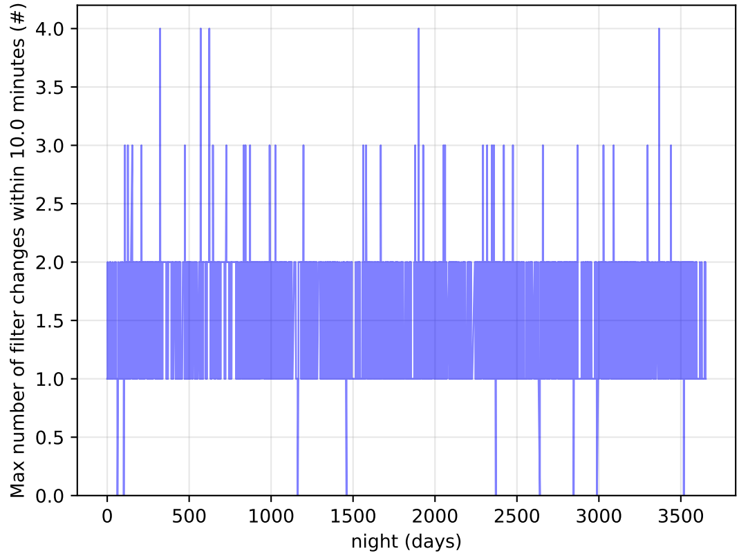
too_elab_r8_d3_griz_v3.4_10yrs Per Night: Max number of filter changes within 10.0 minutes
