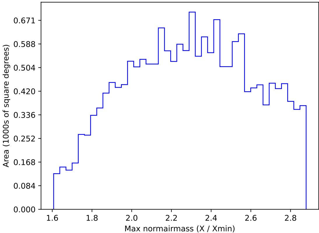
too_elab_r8_d3_griz_v3.4_10yrs WFD z band: Max normairmass
