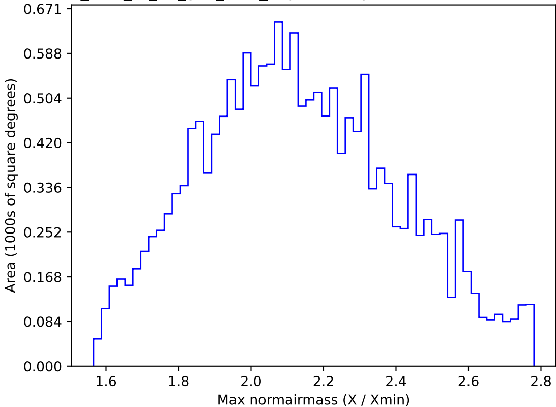
too_elab_r8_d3_griz_v3.4_10yrs WFD y band: Max normairmass
