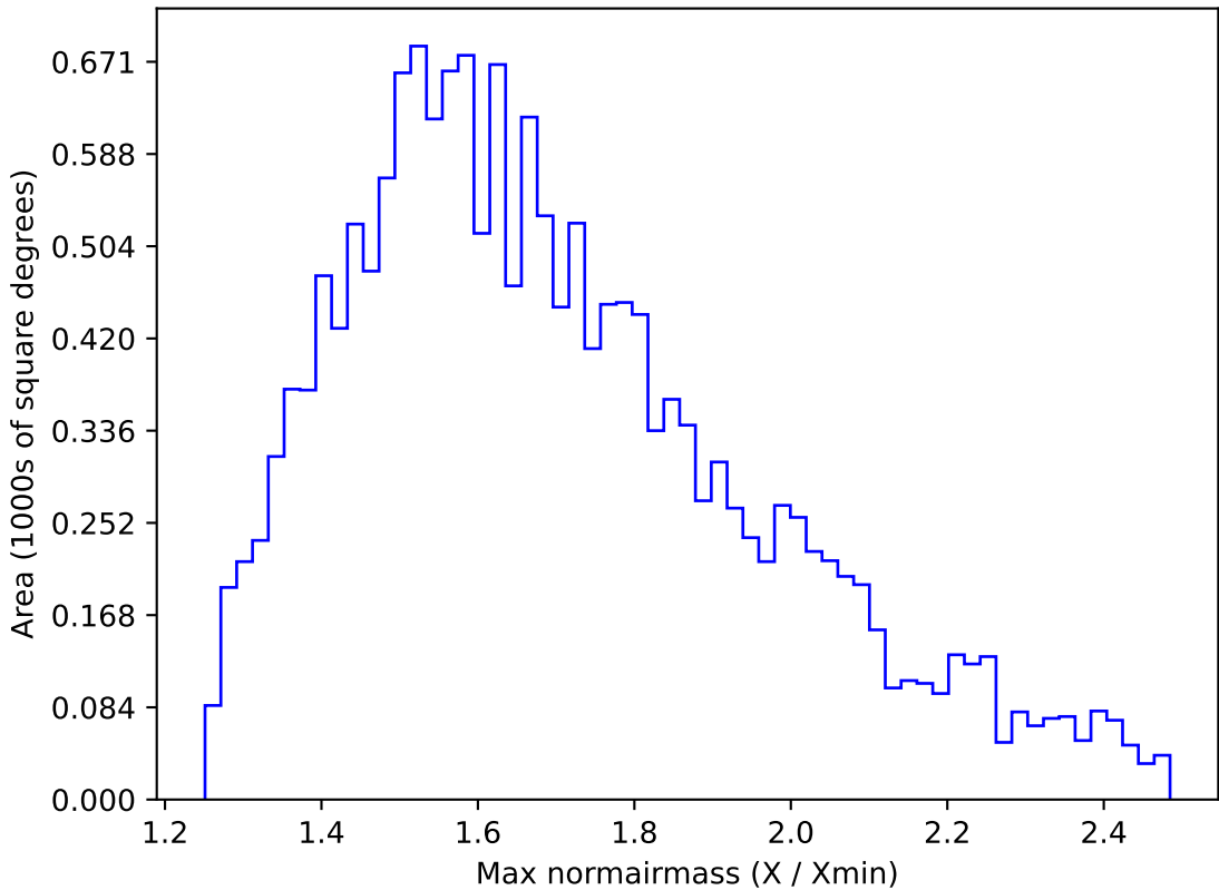
too_elab_r8_d3_griz_v3.4_10yrs WFD u band: Max normairmass
