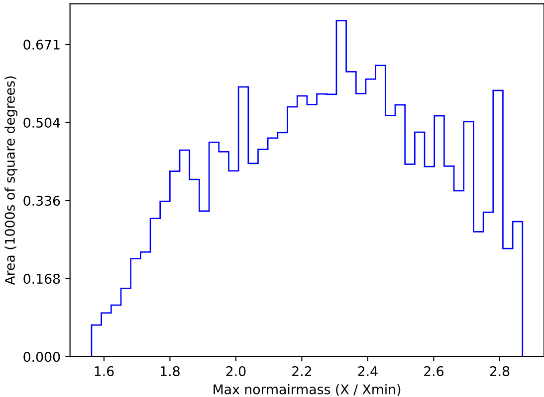
too_elab_r8_d3_griz_v3.4_10yrs WFD i band: Max normairmass
