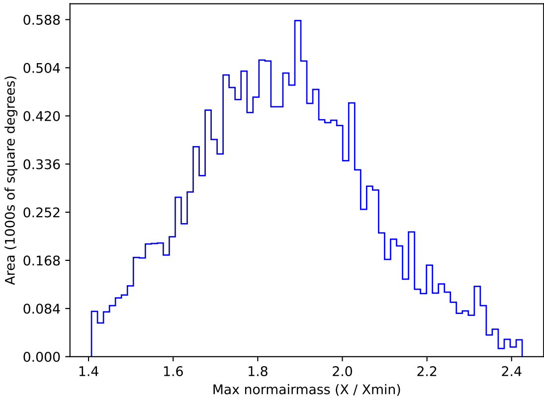
too_elab_r8_d3_griz_v3.4_10yrs WFD g band: Max normairmass
