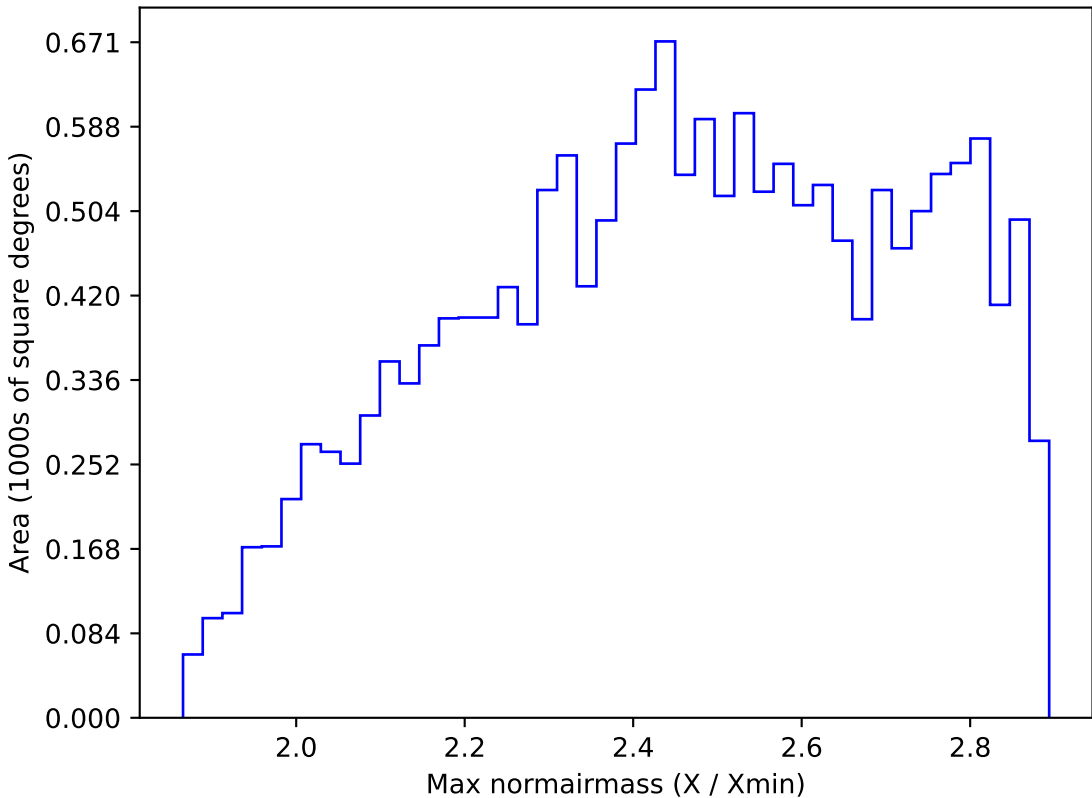
too_elab_r8_d3_griz_v3.4_10yrs WFD all bands: Max normairmass
