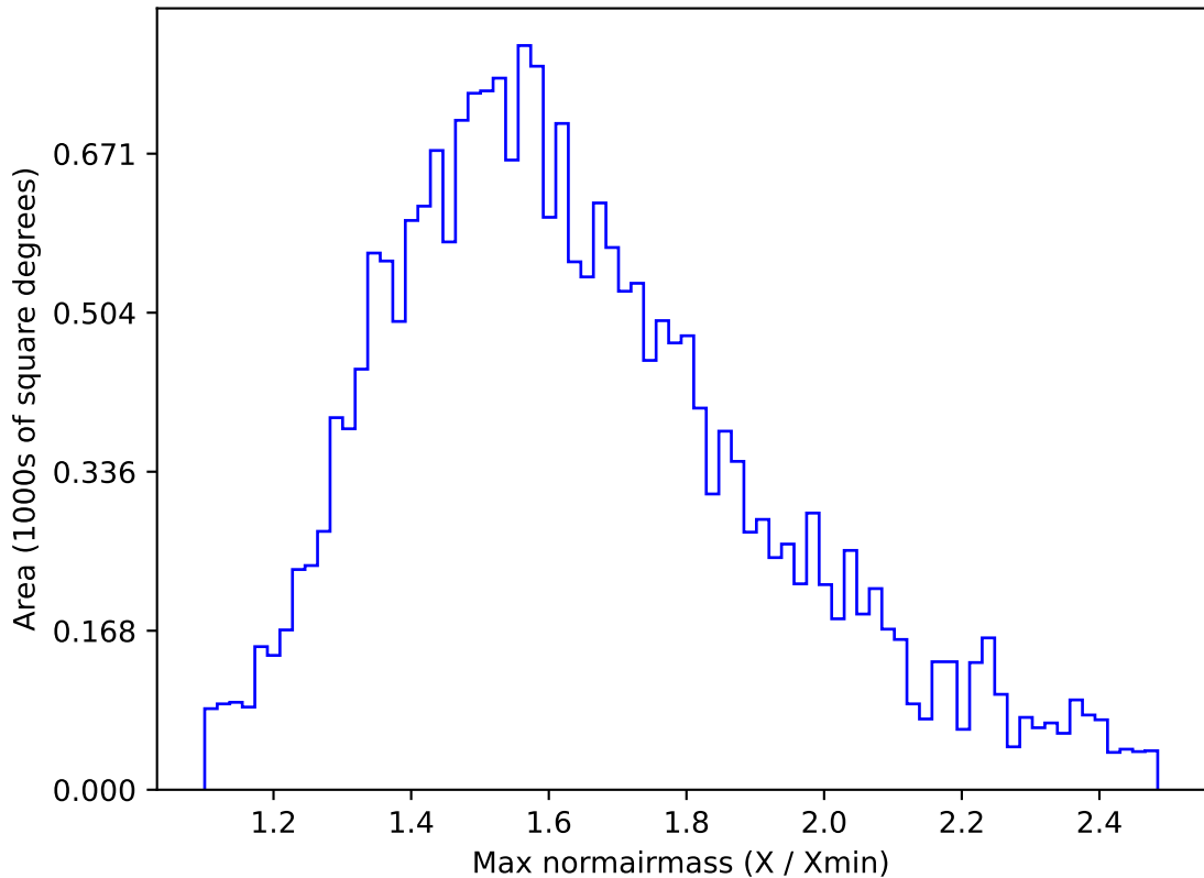
too_elab_r8_d3_griz_v3.4_10yrs All sky u band: Max normairmass
