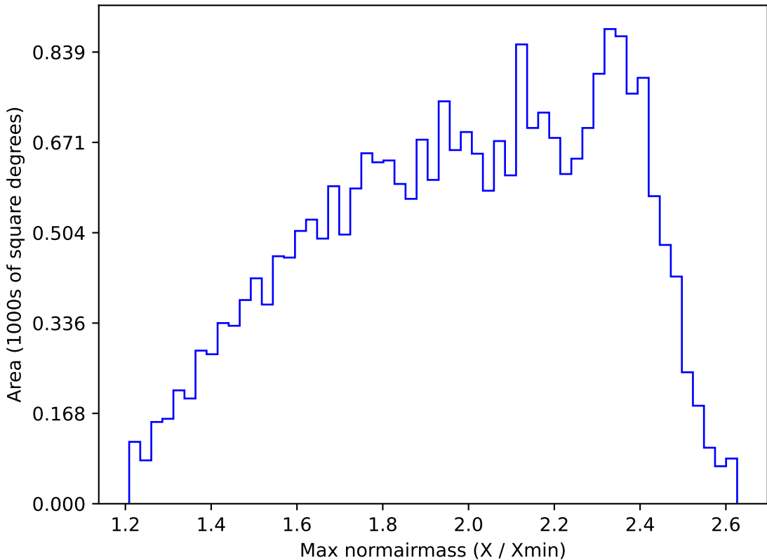
too_elab_r8_d3_griz_v3.4_10yrs All sky r band: Max normairmass
