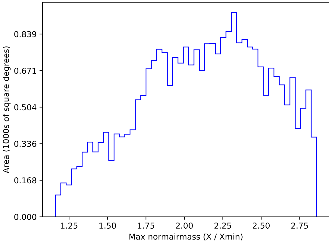
too_elab_r8_d3_griz_v3.4_10yrs All sky i band: Max normairmass
