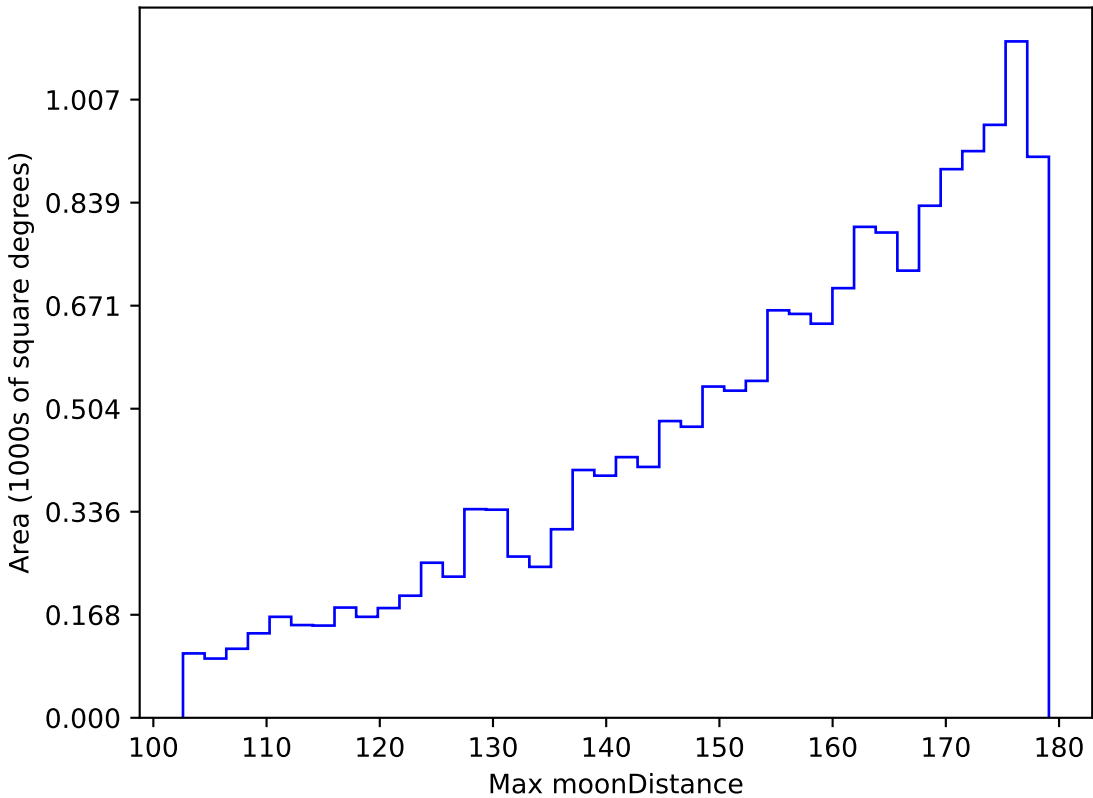
too_elab_r8_d3_griz_v3.4_10yrs WFD z band: Max moonDistance
