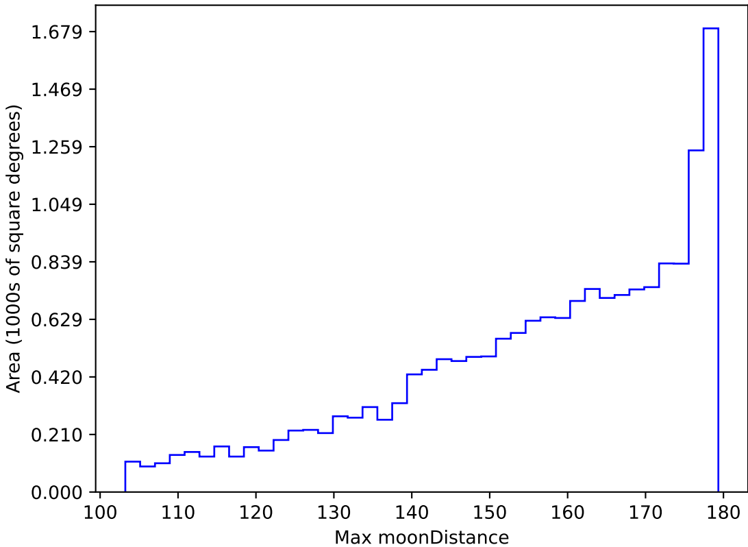
too_elab_r8_d3_griz_v3.4_10yrs WFD r band: Max moonDistance
