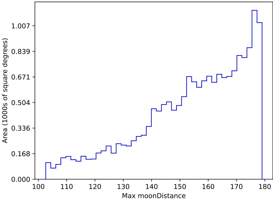
too_elab_r8_d3_griz_v3.4_10yrs WFD g band: Max moonDistance
